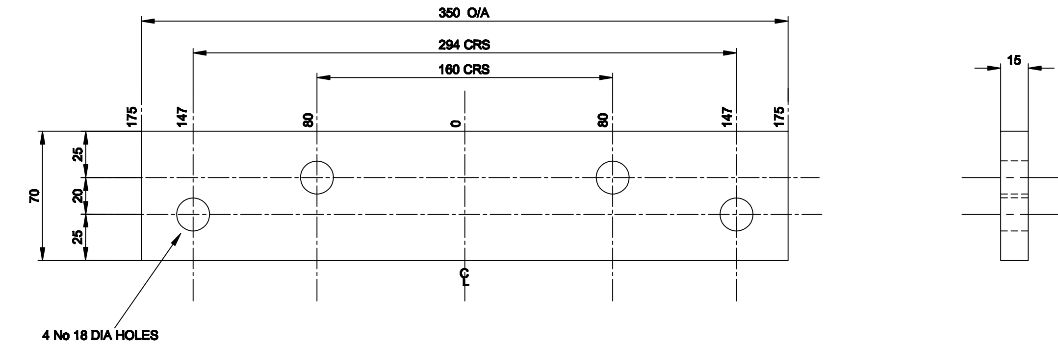
ITEM 10 70 x 15 x 350 LONG - FLAT BAR SCALE 1: 2
