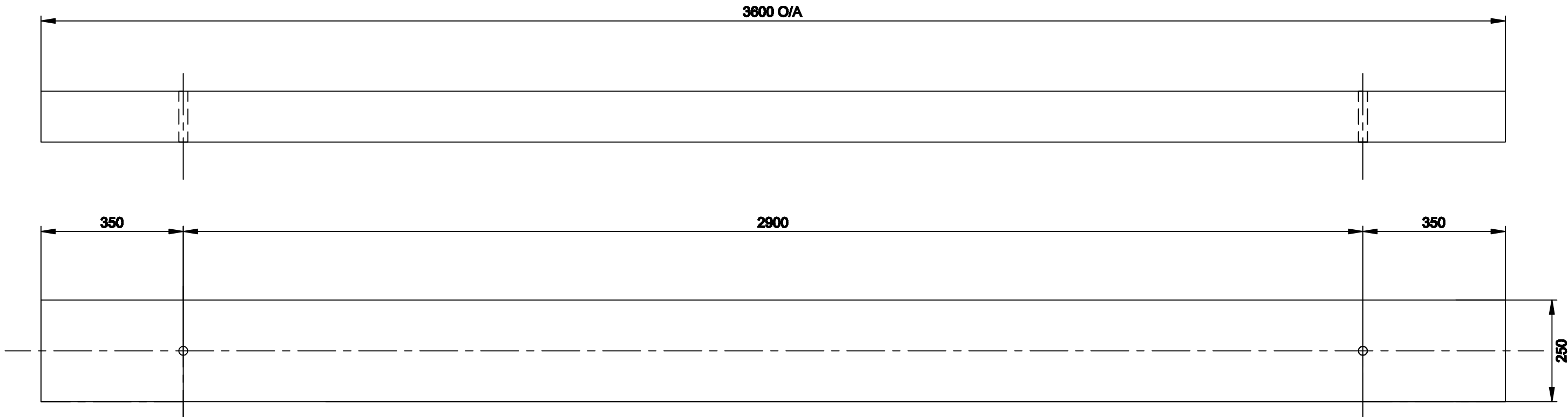
ITEM 8 3600 x 250 x 125 WOOD BAULK SCALE :- 1 : 10
